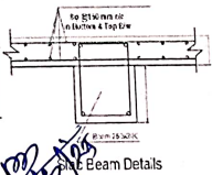
Slab Beam Details
