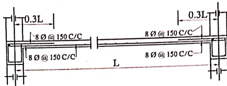
Details Of R.C.C Roof Slab & Beam
