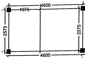
LAYOUT PLAN
