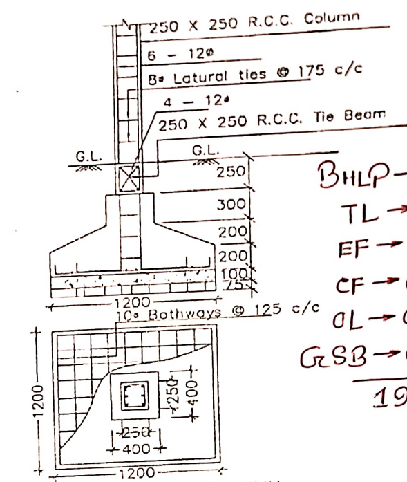
DETAILS OF R. C. C COLUMN (SCALE - 1 : 25)
