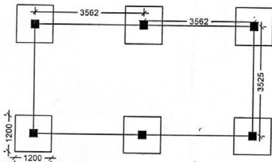
LAYOUT PLAN
