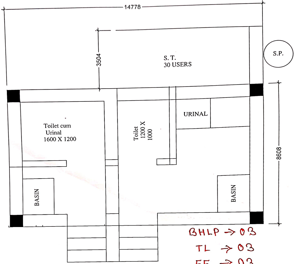
PLAN
