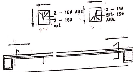
Details Of R.C.C Roof Slab & Beam (SCALE - 1 : 25)
