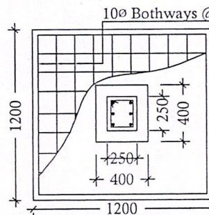
DETAILS OF R. C. C COLUMN
