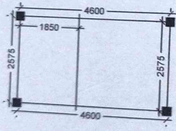
LAYOUT PLAN
