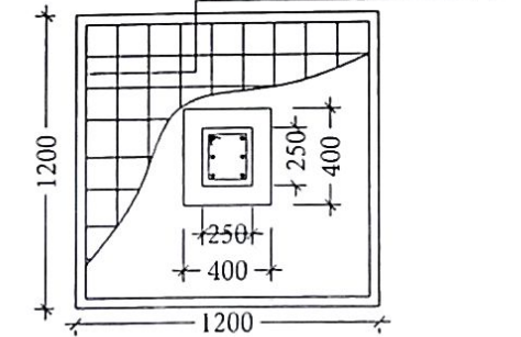
DETAILS OF R. C. C COLUMN (SCALE - 1 : 25)
