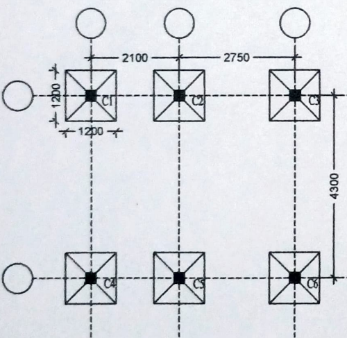
FOOTING LAYOUT
