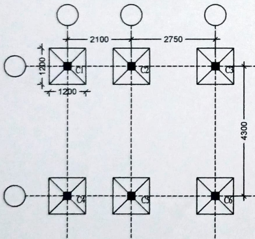
FOOTING LAYOUT
