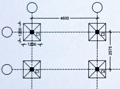
FOOTING LAYOUT
