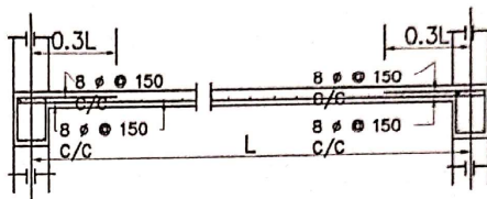
Details Of R.C.C Roof Slab & Beam (SCALE - 1 : 25)
