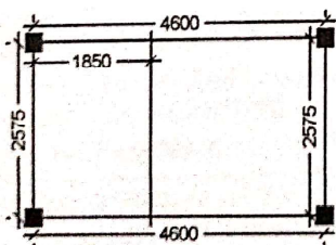
LAYOUT PLAN
