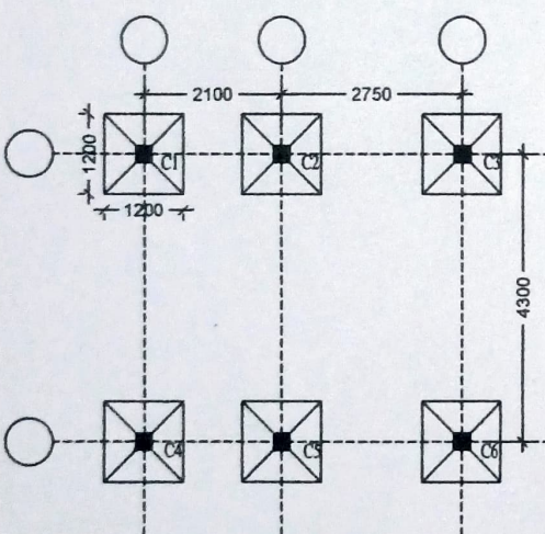
FOOTING LAYOUT
