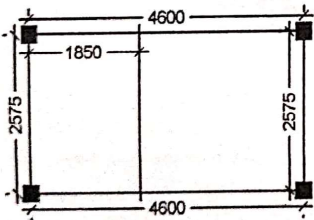
LAYOUT PLAN
