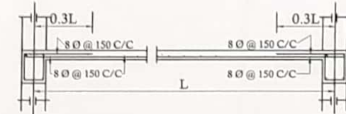
Details Of R.C.C Roof Slab & Beam
