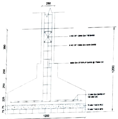
CROSS SECTION OF RCC FOUNDATION (1:25)
