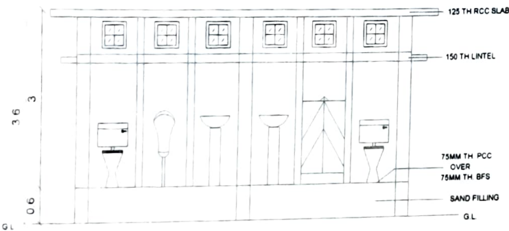
CROSS SECTIONAL VIEW AT X-Y
