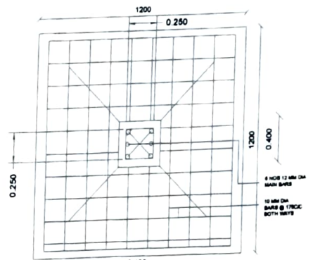
PLAN OF RCC FOUNDATION (1:25)
