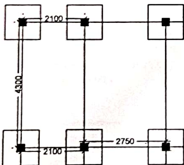
LAYOUT PLAN
