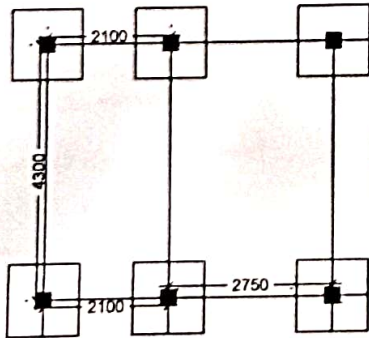
LAYOUT PLAN
