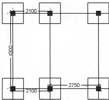
LAYOUT PLAN
