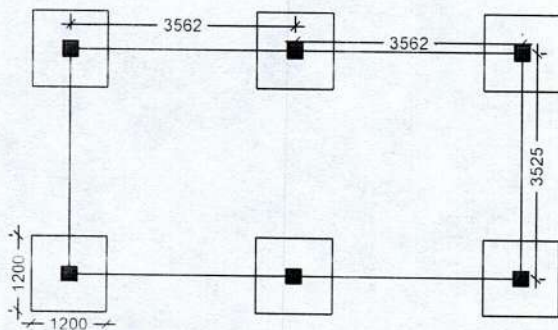
LAYOUT PLAN
