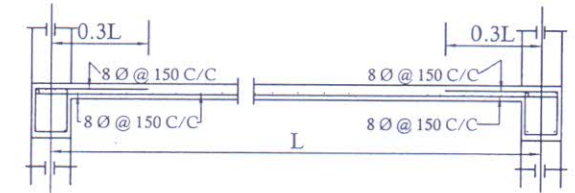
Details Of R.C.C Roof Slab & Beam (SCALE - 1 : 25)
