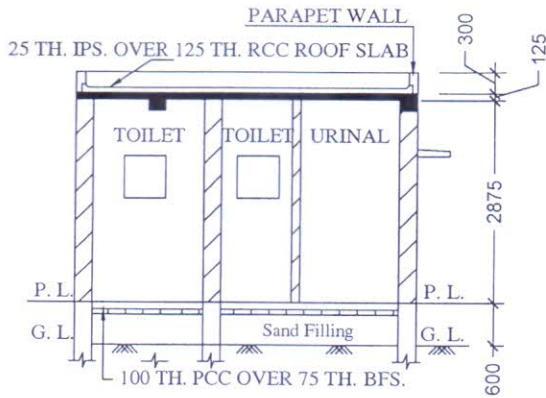
FRONT ELEVATION
