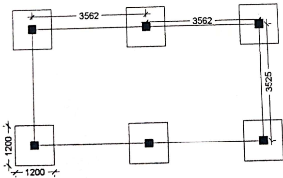
LAYOUT PLAN
