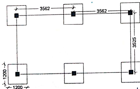
LAYOUT PLAN
