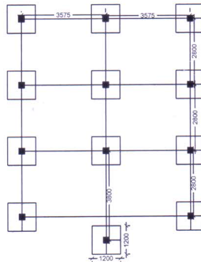
LAYOUT PLAN
