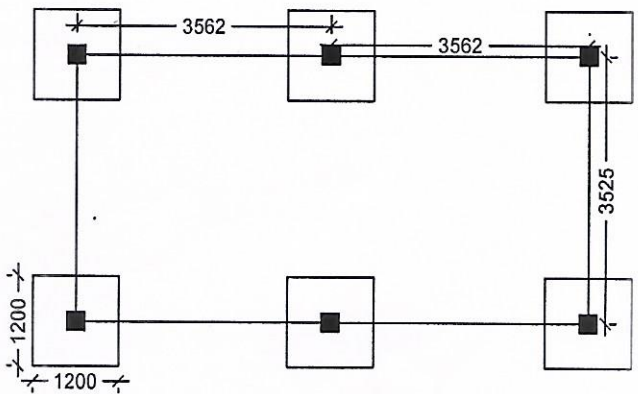
LAYOUT PLAN
