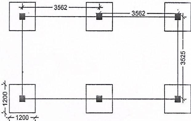
LAYOUT PLAN
