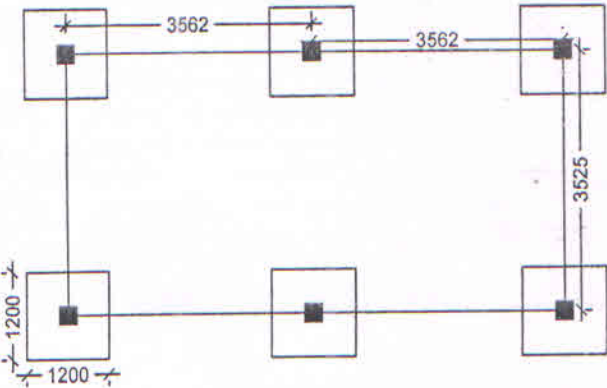
LAYOUT PLAN
