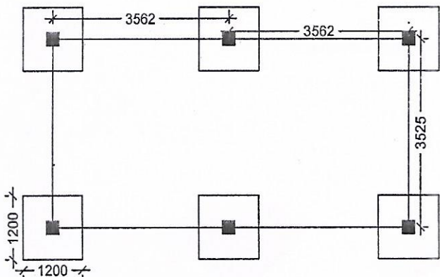
LAYOUT PLAN
