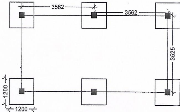
LAYOUT PLAN
