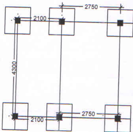
LAYOUT PLAN
