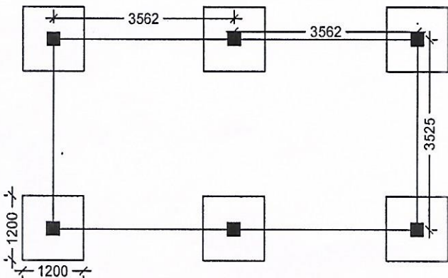
LAYOUT PLAN
