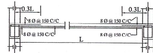
Details Of R. C. C Roof Slab & Beam (SCALE - 1 : 25)
