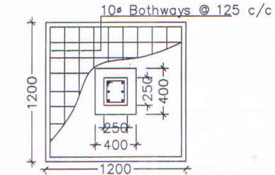
DETAILS OF R. C. C COLUMN
