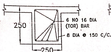
DETAILS OF BEAM AT MID SPAN
