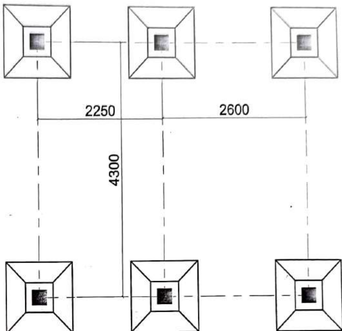
COLUMN LAYOUT PLAN
