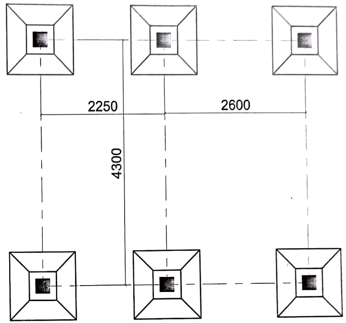
COLUMN LAYOUT PLAN COLUMN 250x250
