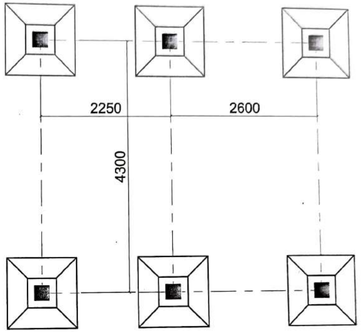
COLUMN LAYOUT PLAN COLUMN 250x250
