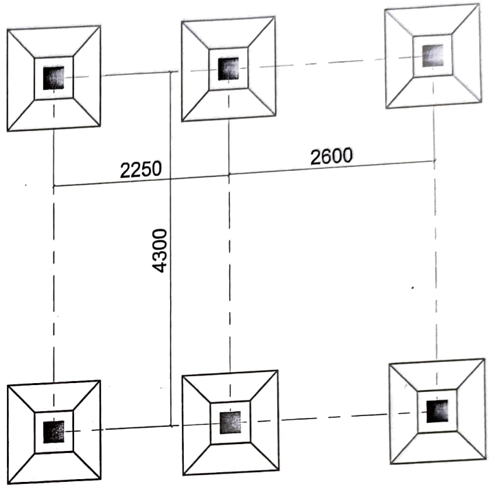
COLUMN LAYOUT PLAN COLUMN 250x250
