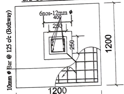
PLAN OF FOOTING COLUMN 250x250 SCALE 1:30
