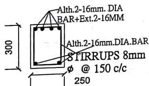
AT SUPPORT SEC. ON SLAB BEAM SCALE 1:25
