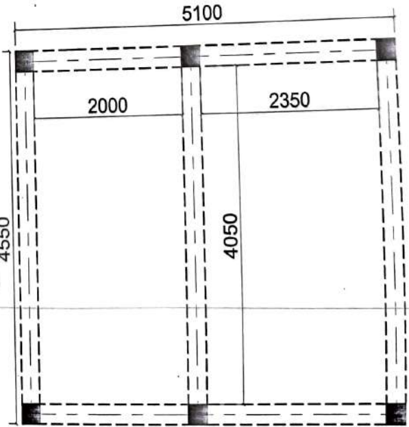
TIE & FLOOR BEAM PLAN
