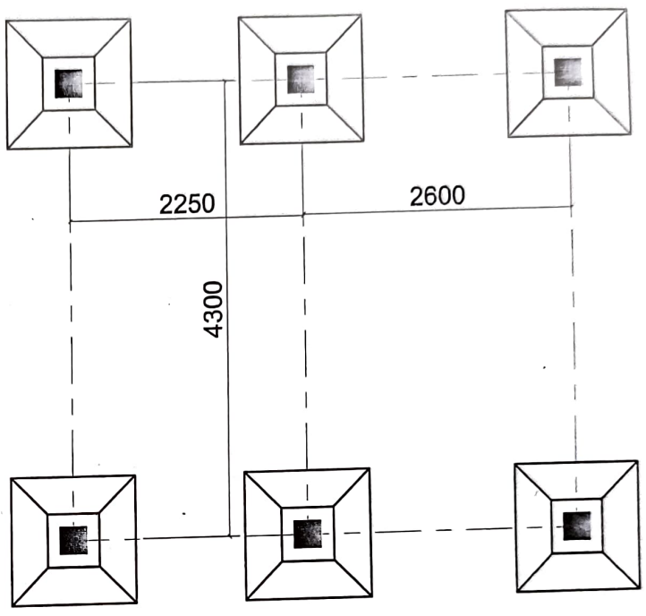
COLUMN LAYOUT PLAN COLUMN 250x250
