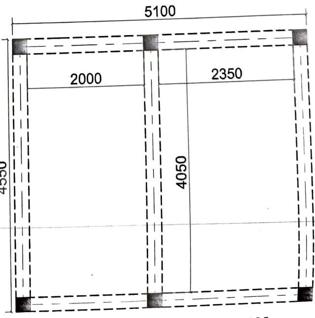
TIE & FLOOR BEAM PLAN
