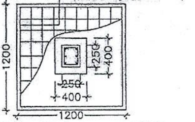
DETAILS OF R. C. C COLUMN (SCALE - 1 : 25)
