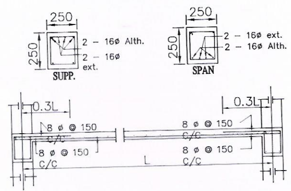
Details Of R.C.C Roof Slab & Beam (SCALE - 1 : 25)
