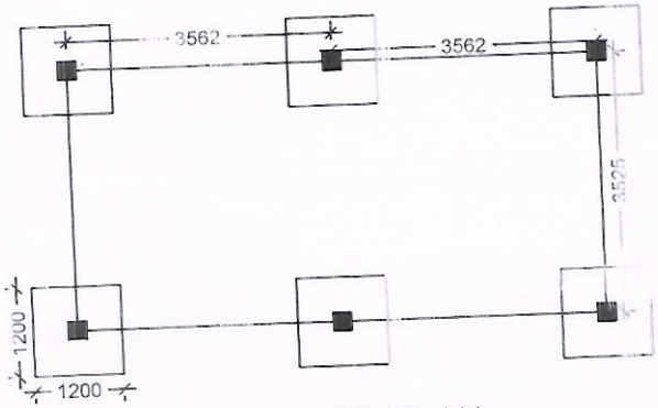
LAYOUT PLAN
