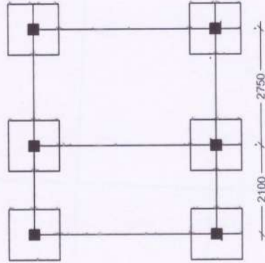
LAYOUT PLAN
