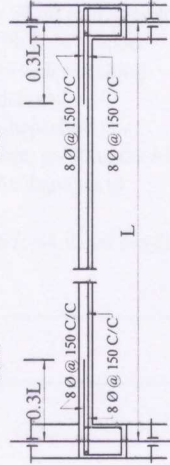
Details Of R.C.C. Roof Slab & Beam
