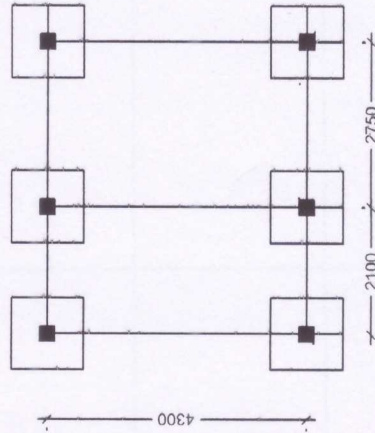
LAYOUT PLAN
