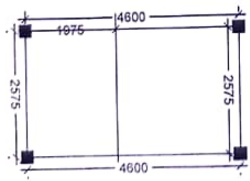
LAYOUT PLAN
